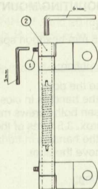
Illustration of hinge
