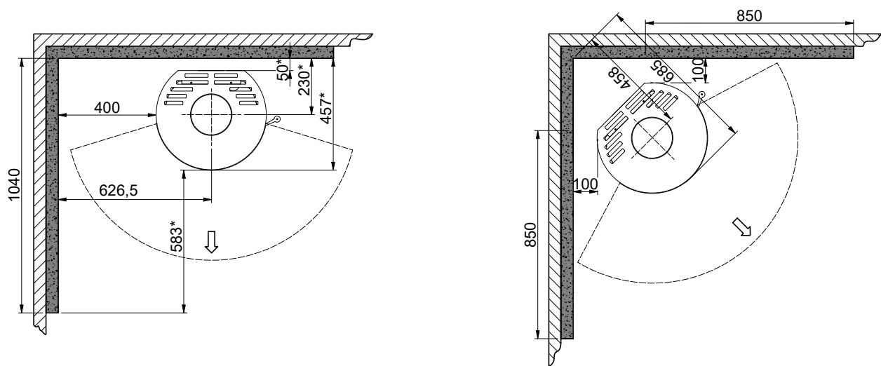
Minimum distance to flammable wall protected by a fire wall
