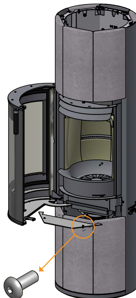
2 pcs. M5x12 RH socket head cap screws
